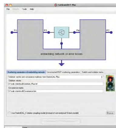
Fig. 13: The CalibratedDUT Plus tool from the NIST Uncertainty Framework package
